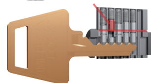
Reverse rake tapered driver pin
